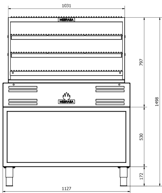
VISTA FRONTAL
