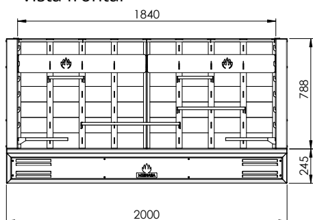
Vista frontal
