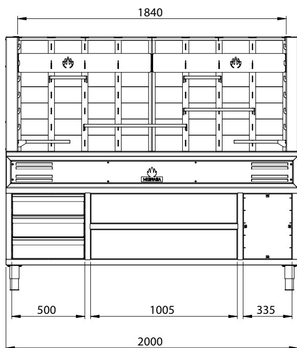
VISTA FRONTAL
