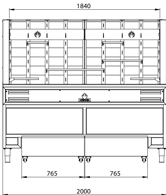
VISTA FRONTAL
