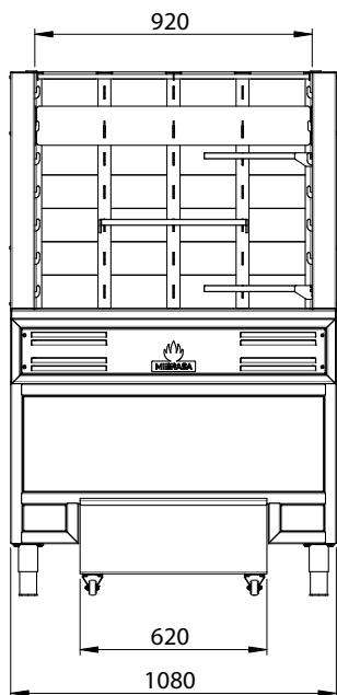
VISTA FRONTAL
