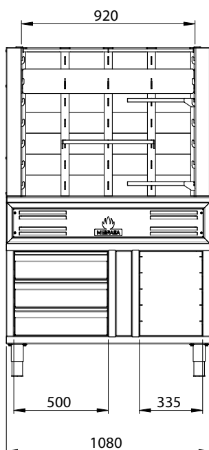
VISTA FRONTAL
