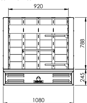
Vista frontal
