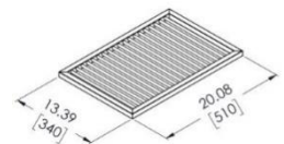
Parrilla heating rack (x2)
