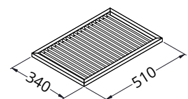
DIMENSION DE SUPPORT PLATEAUX
