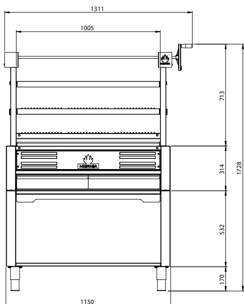
VISTA FRONTAL
