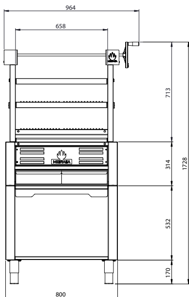
VISTA FRONTAL
