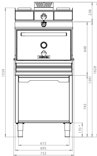
Vista frontal
