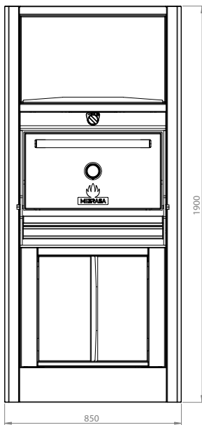
Vista frontal
